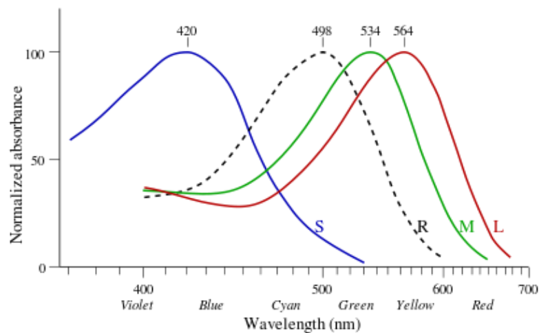
Normalised absorption spectra of the three human photopsins and of human rhodopsin (dashed).
